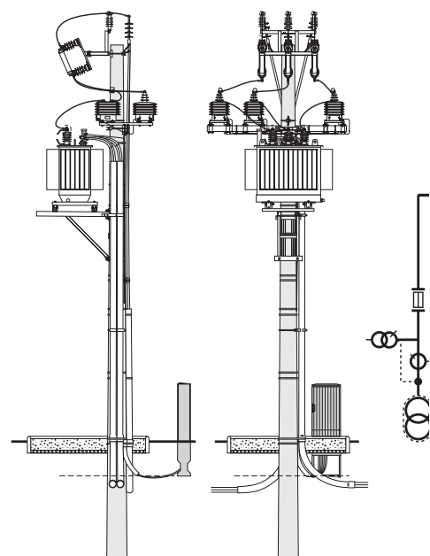
STSRS - 20/630-KK2-9,0/10-P3
