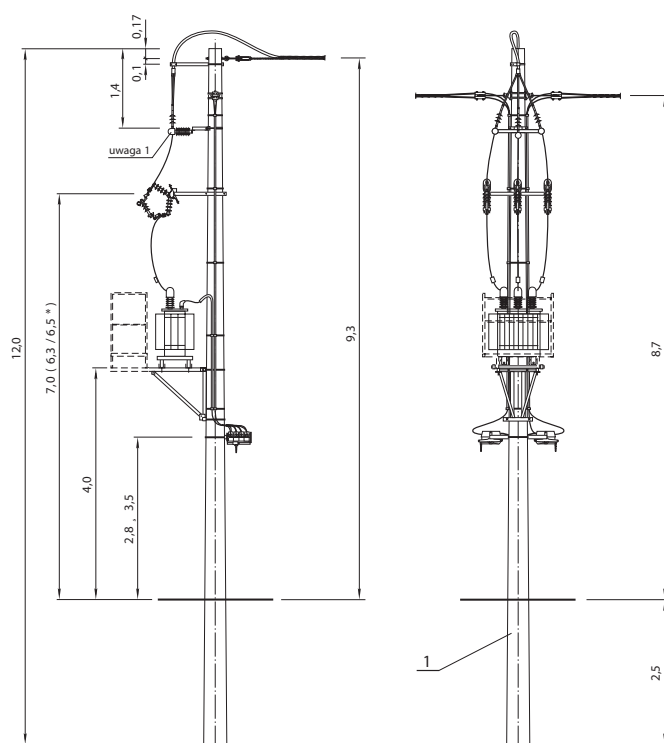
STNKs-20/□/II, STNKp-20/□/II
