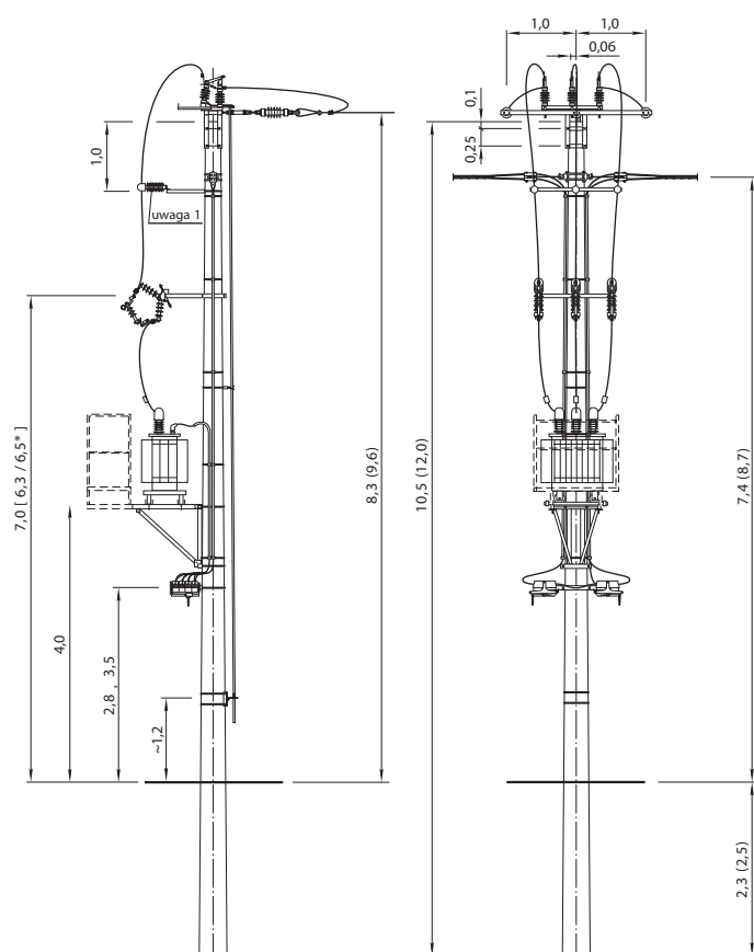
STNo-20/□
