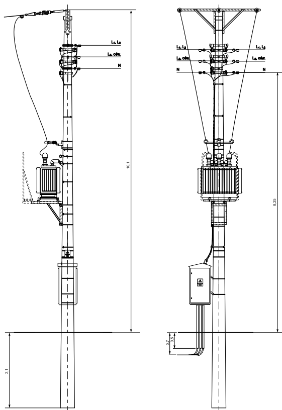
STSRu - 20/250 - Wariant II
